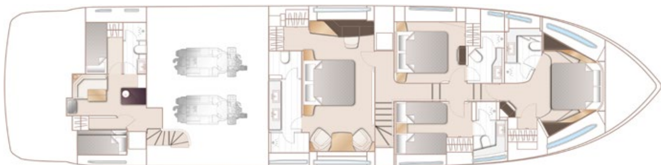
LOWER DECK
